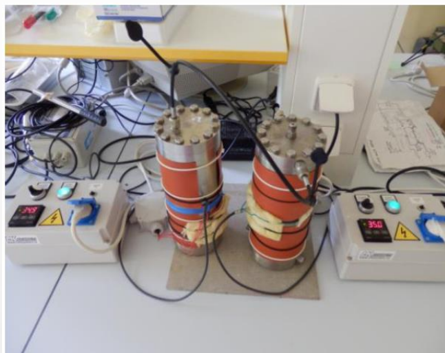
Photo of the apparatus used for long-term static experiments - REPP-CO 2 (UJV, CGS)
