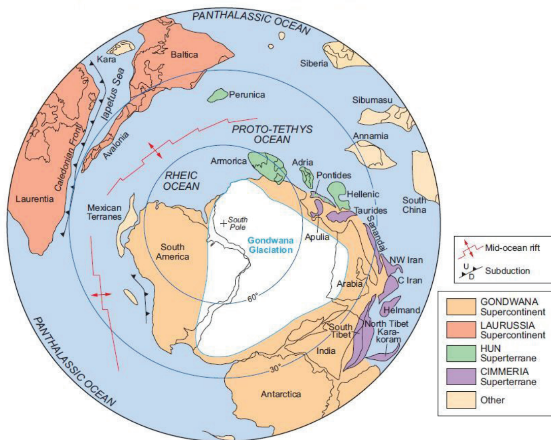
Figure 2. Paleogeography of the boundary of the Uppermost Ordovician and Lowermost Silurian (before 440 Ma). Ruban, D.A. – Al-Husseini, M.I. – Iwasaki, Y. (2007).
